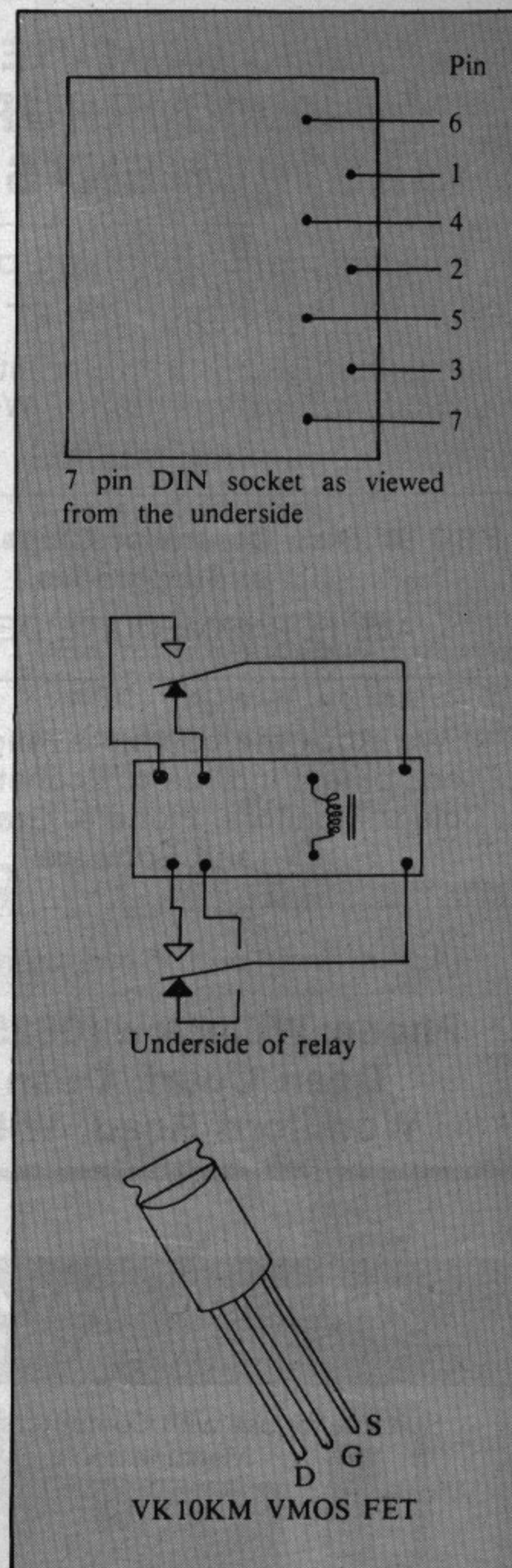
Figure IX: Component pinout
